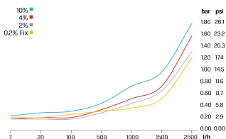
Pressure Loss
